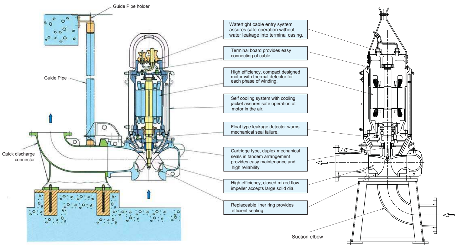
DSC3 : WET PIT INSTALLATION
